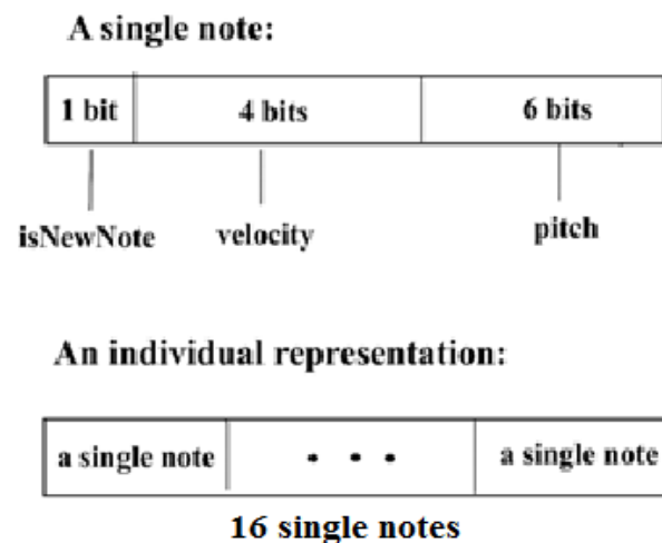
Figure 1: Representation for a single music note and an individual
