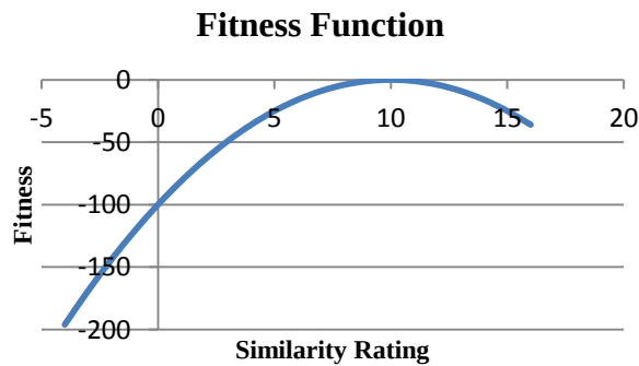
Figure 4: Fitness function: f(x) = -(x-10)^2 . Input is a similarity rating.
