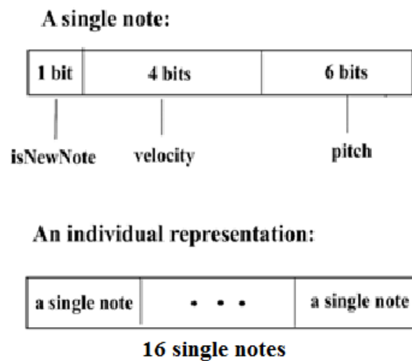
Figure 9: Representation for a single music note and an individual
