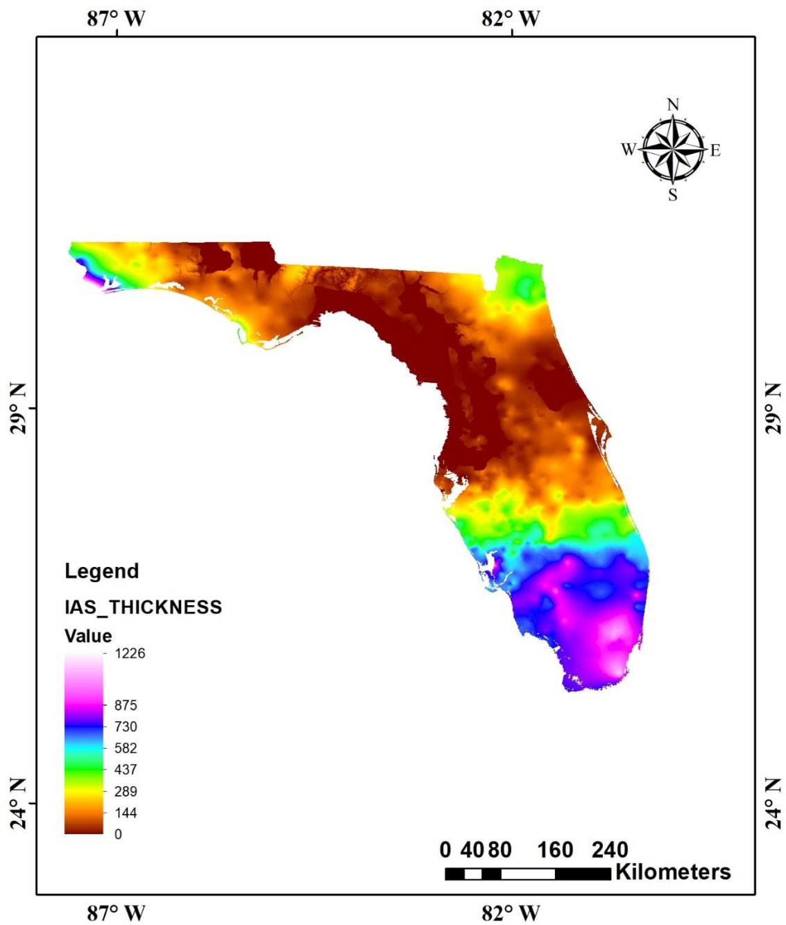
Figure 4. Thickness range of the Intermediate Aquifer System (IAS) across the state of Florida.
