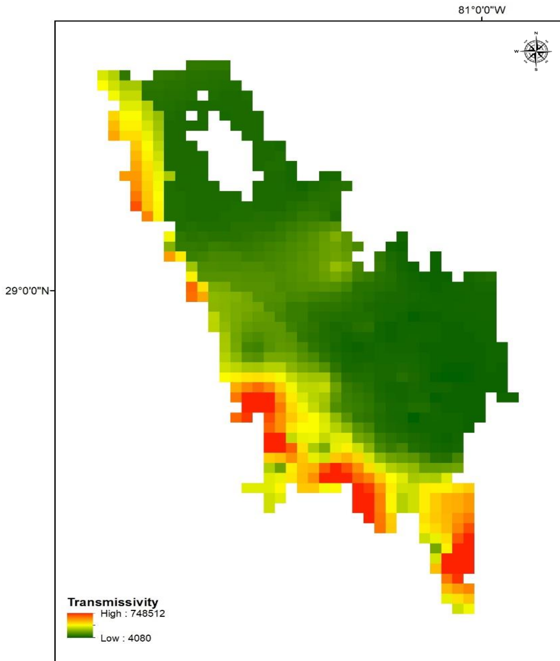
Figure 15. Interpolated transmissivity based on interpolation of ~1500 aquifer test of the Upper Floridan Aquifer, in units of feet squared per day.
