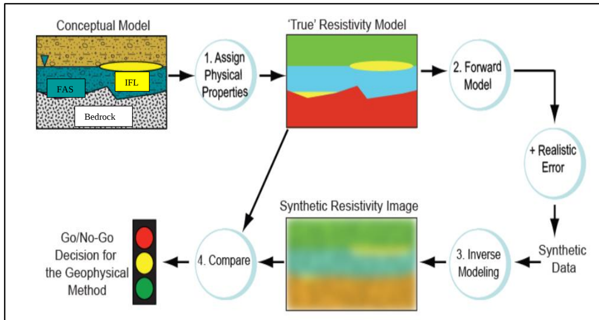
Figure 18. Pre-modeling workflow done within ResIPy software.
