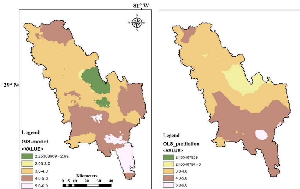
Figure 21. Left to right: GIS model observation and OLS geostatistical predictions.
