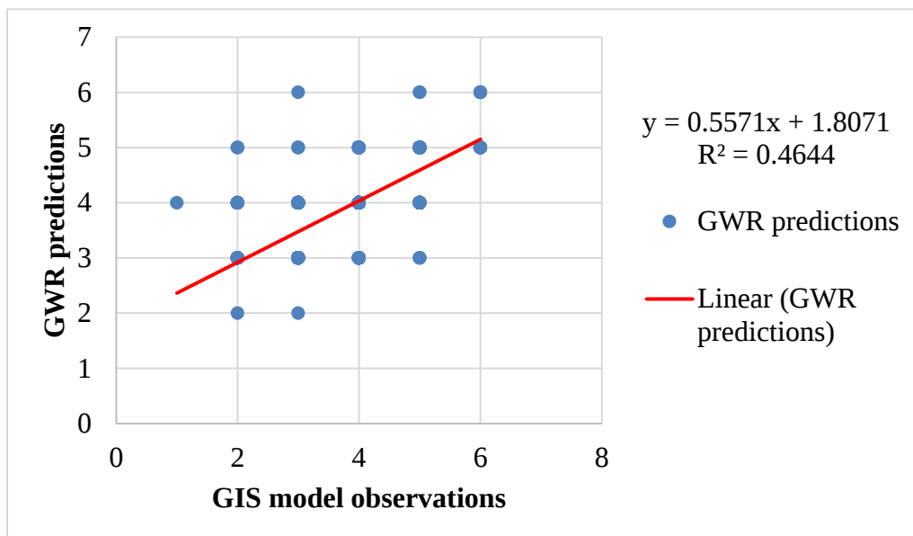
Figure 24. Relationship between GIS model observation and GWR geostatistical prediction.
