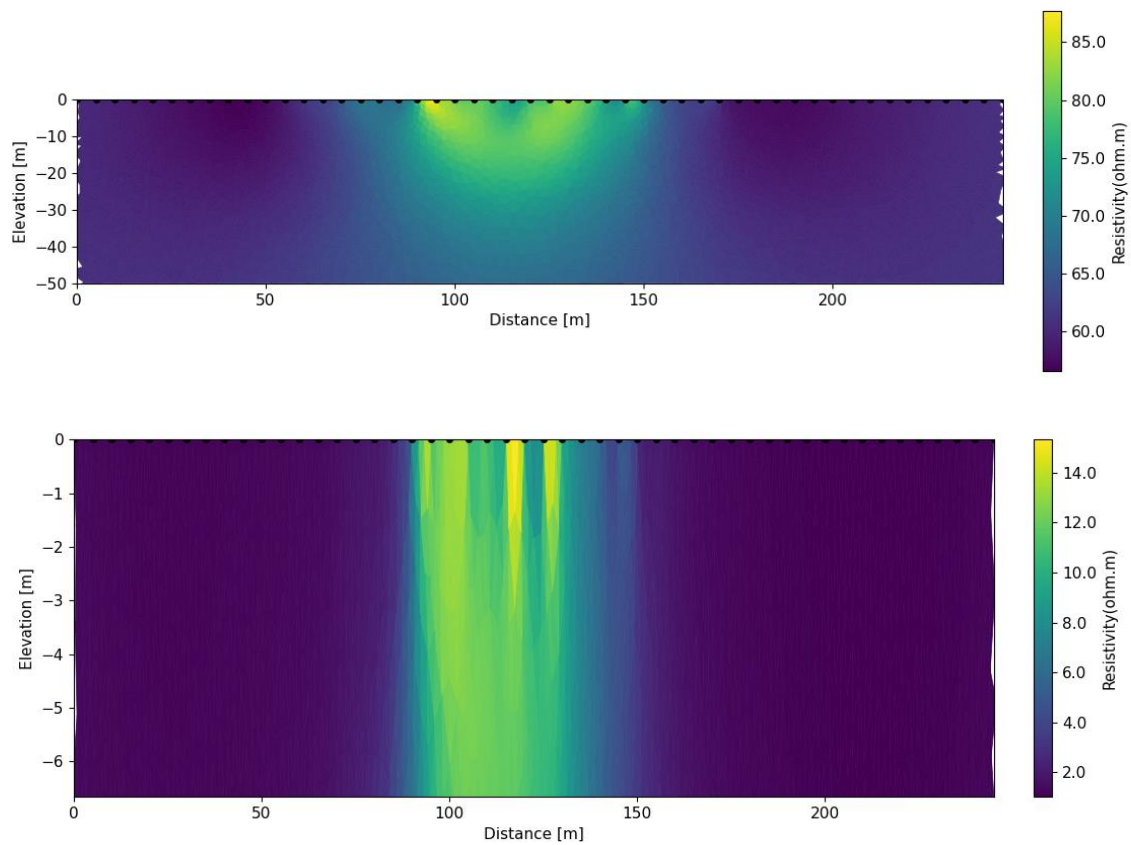
Figure 32. Inverted true resistivity values for water classes for dipole-dipole (top) and Wenner array (bottom).
