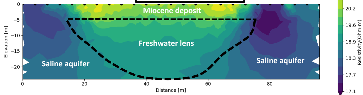
Figure 33. Wenner configuration on part of the Geneva lens (model is not drawn to scale).
