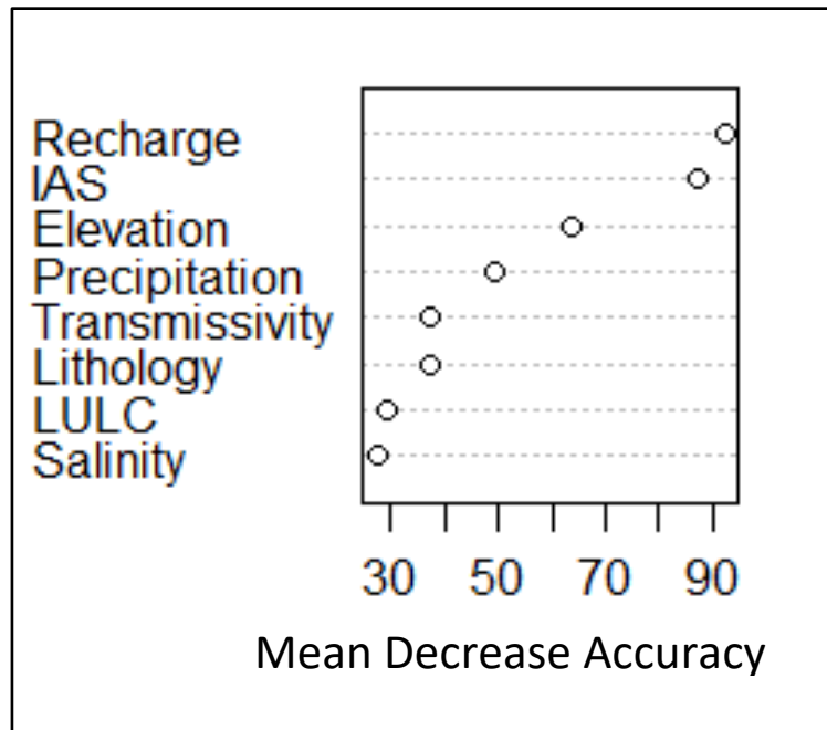
Figure 26. Variable importance derived from the RF model.
