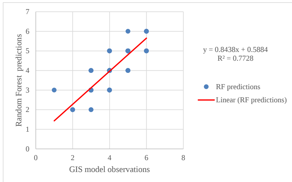
Figure 29. Relationship between GIS model observation and machine learning algorithm, RF predictions.
