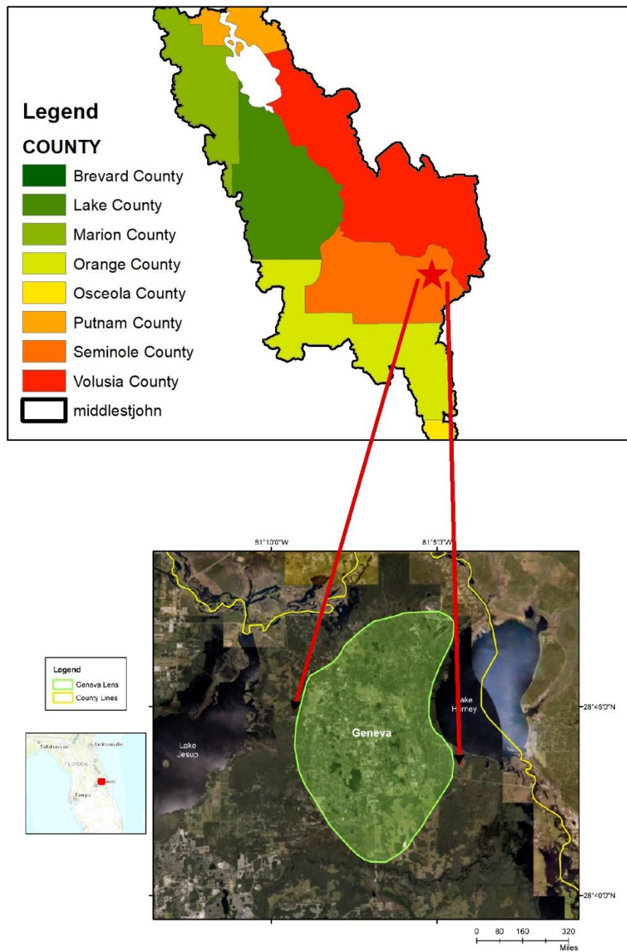
Figure 6. The areal extent of the Geneva lens located within the Middle St. Johns watershed, juxtapose Lake Jesup and Lake Harney.
