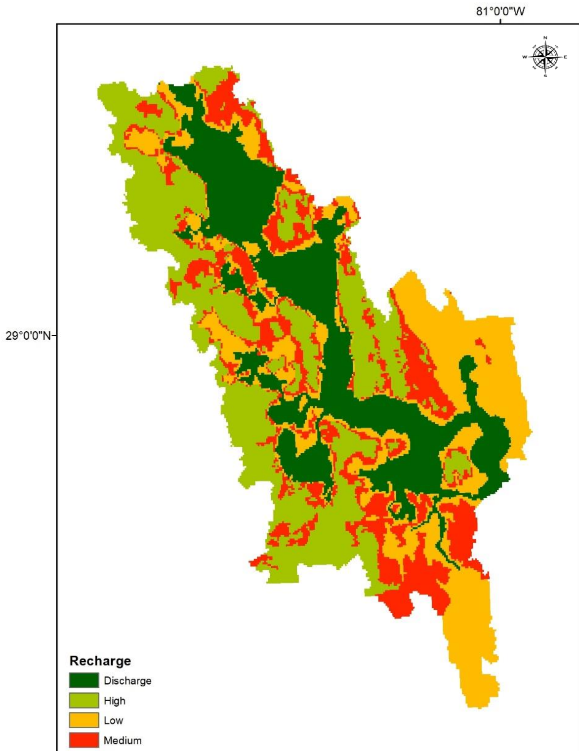
Figure 12. Recharge zones classes to the upper Floridan aquifer.
