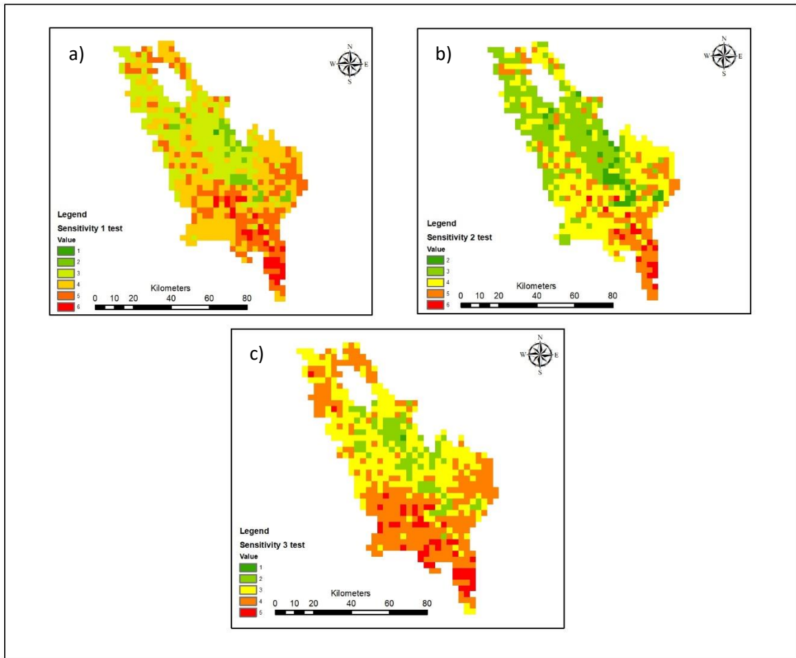
Figure 16. Weight Overlay Index Analysis sensitivity test.
