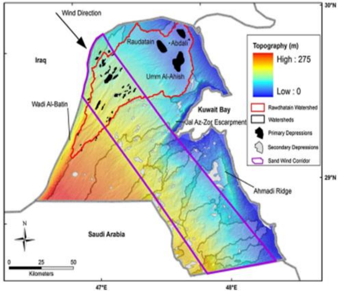
Figure 2. Topographically induced depressions identified in Kuwait. Primary depressions are suggestive areas of untapped groundwater within the Raudhatain watershed.
