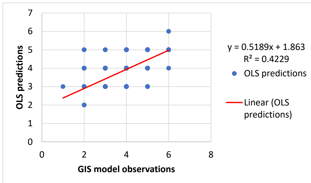
Figure 22. Relationship between GIS model observations and OLS geostatistical predictions.
