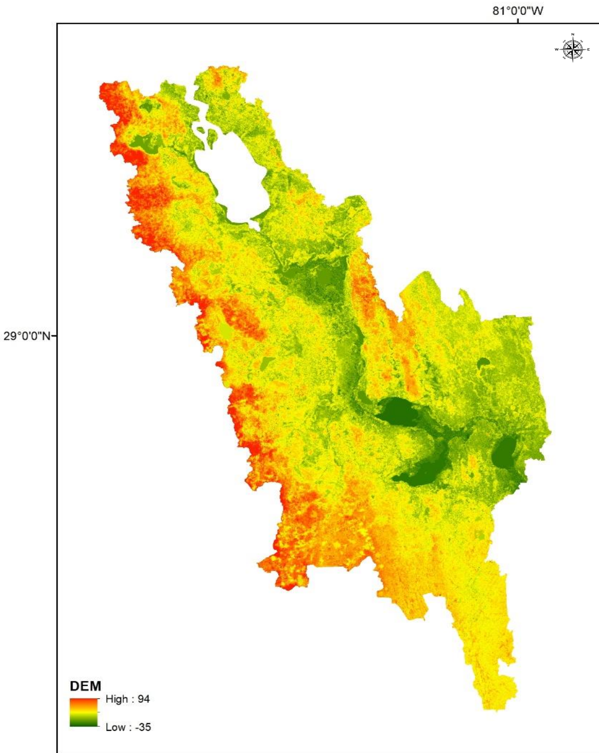
Figure 9. Digital elevation model (DEM) showing elevations in feet.
