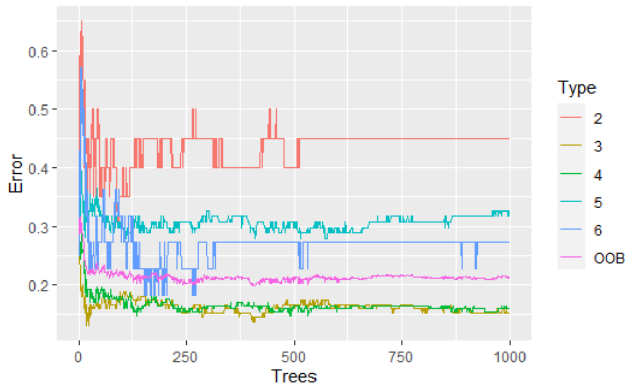
Figure 25. Optimization number of trees bases on OOB estimates of the error rate in the RF model.
