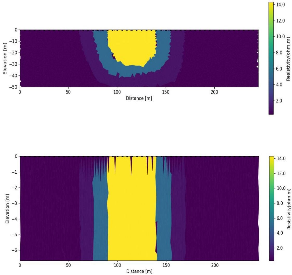
Figure 31. Modeled resistivity values assigned to water classes as they relate to a one-dimensional and homogenous Earth. The top image shows the model used for the dipole-dipole array and the bottom image shows the model used for the Wenner array.
