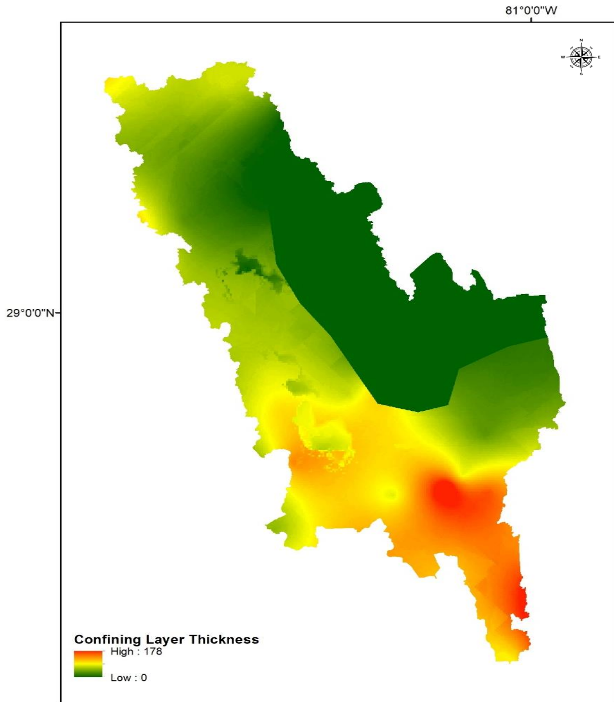
Figure 11. Variable confinements of the hydrostratigraphic unit of the intermediate aquifer system.
