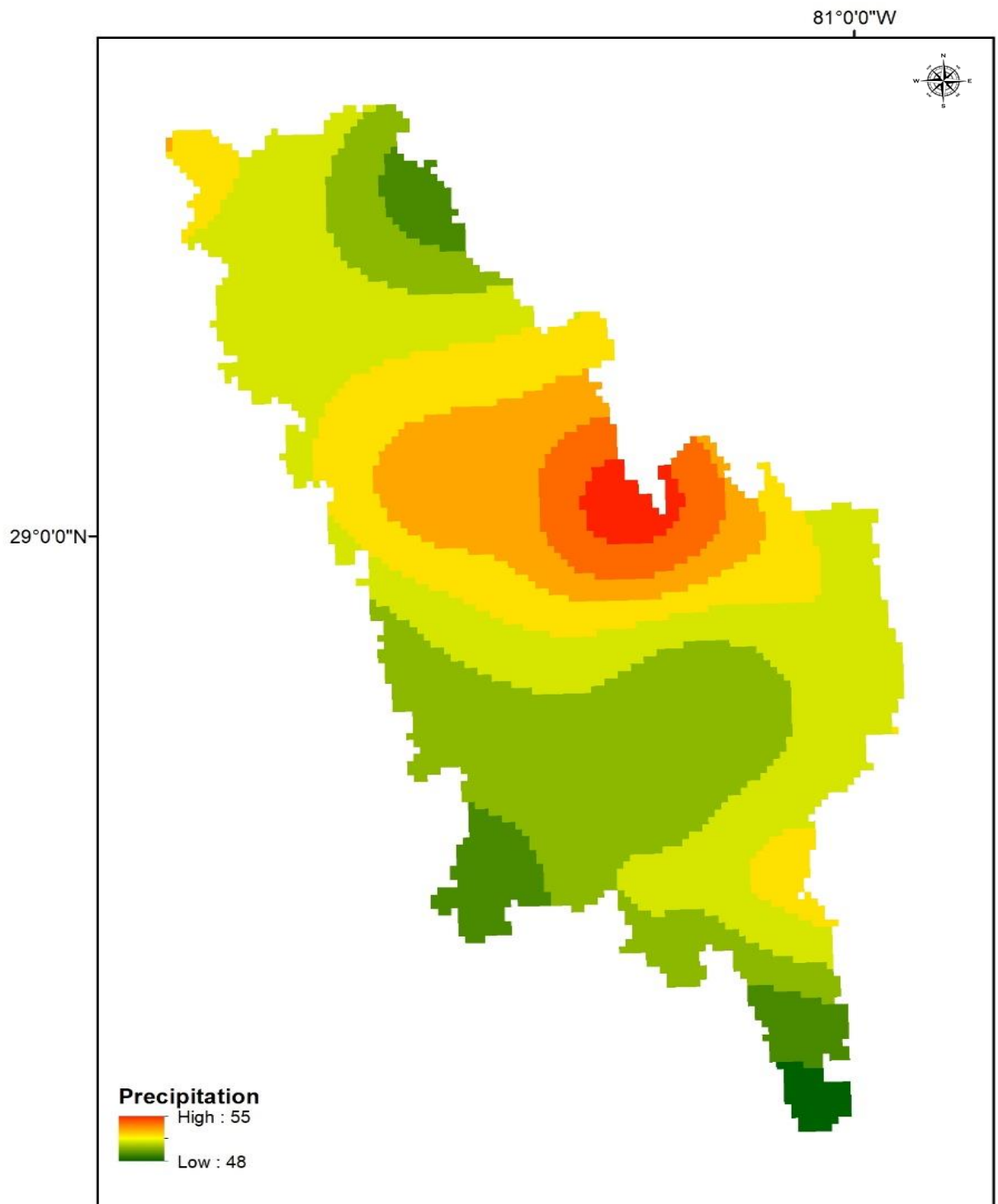
Figure 8. High-resolution 30-year average (1981-2010) precipitation data.
