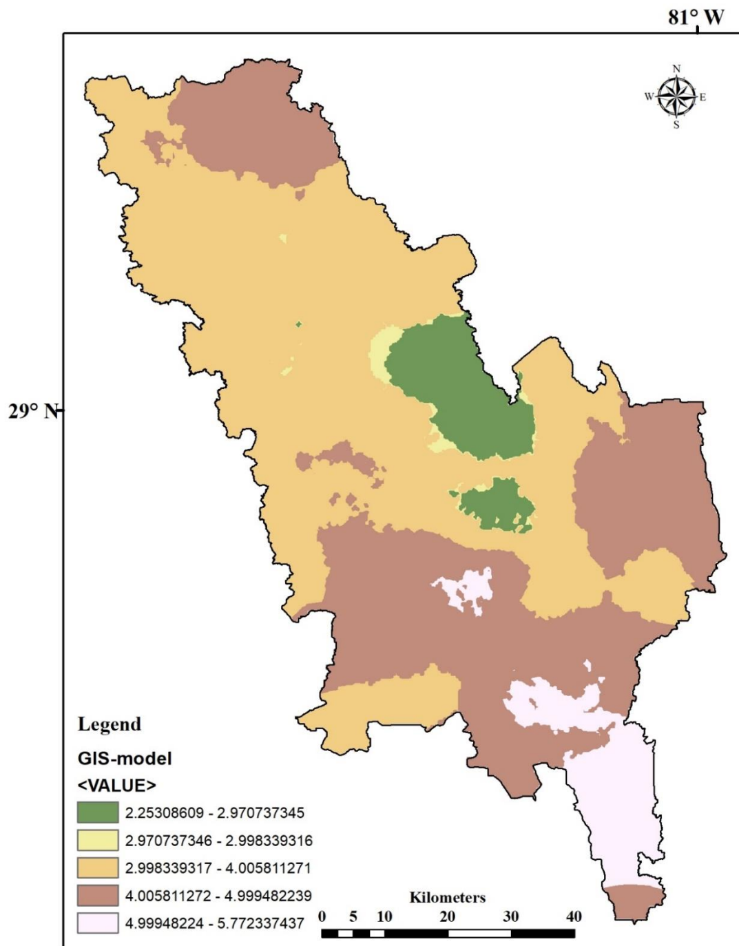
Figure 20. GIS-data driven model output for IFL potential zones within the Middle St. Johns watershed. Areas in green marks areas for low, orange for moderate, and pink for high potential zones.
