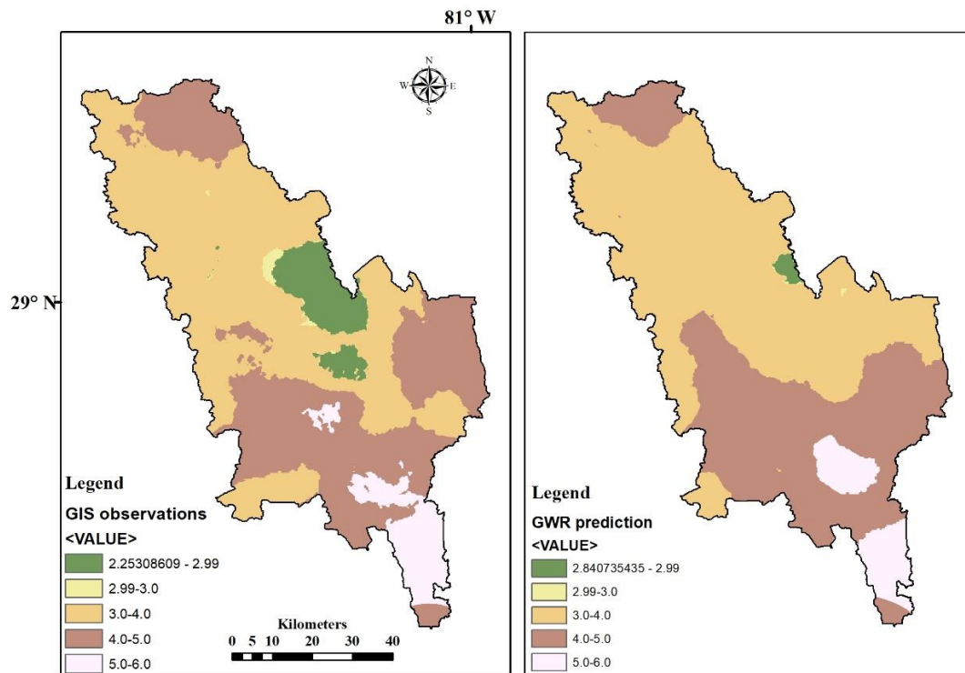
Figure 23. Left to right: GIS model observations and GWR geostatistical predictions.
