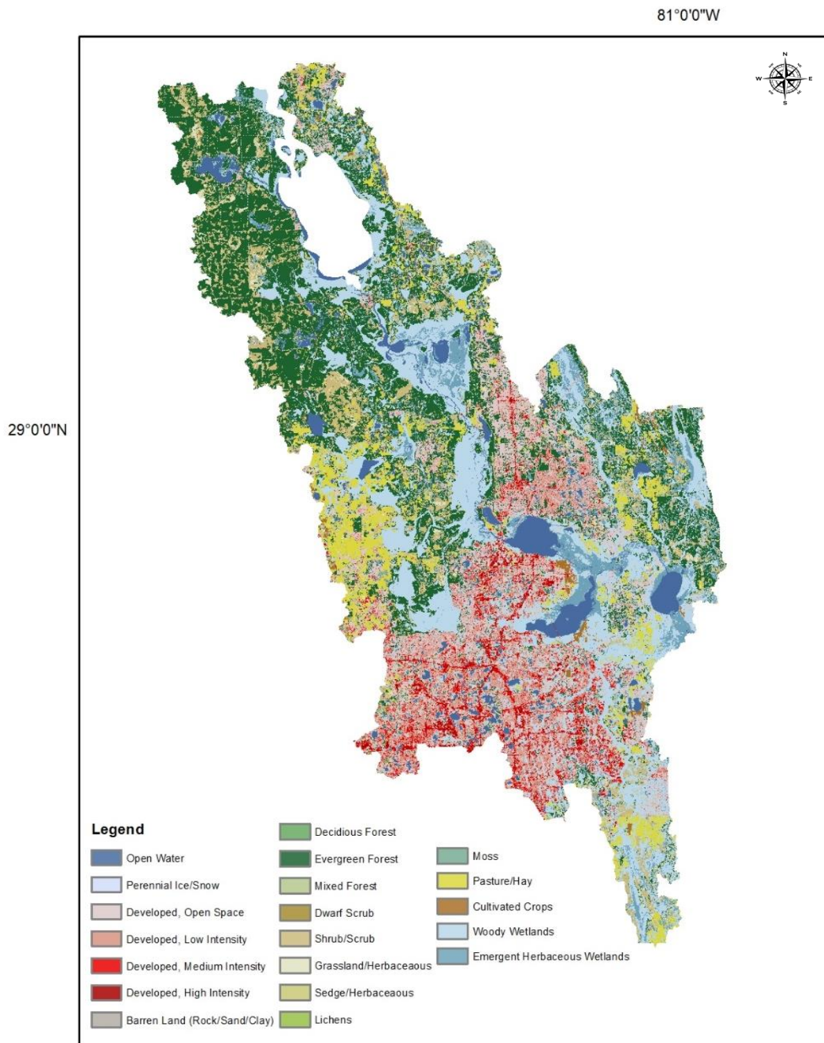
Figure 13. National land cover database 2011 (NLCD2011)
