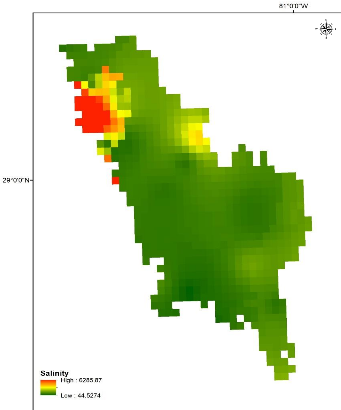
Figure 10. Interpolated total dissolved solids (TDS) concentration, milligrams per liter for the top 50 feet of the Floridan aquifer system for the top 50 feet of the Floridan aquifer system.
