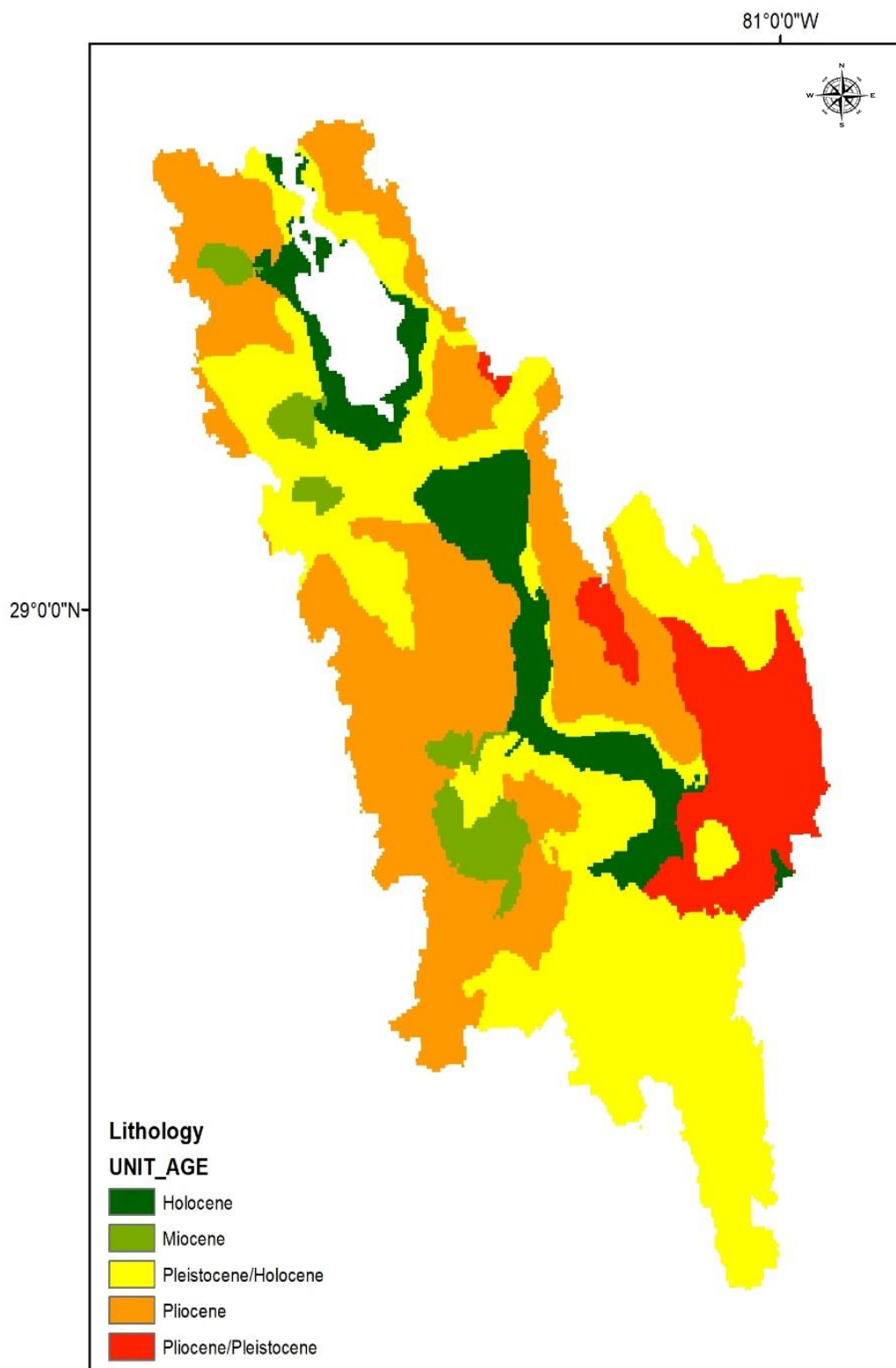
Figure 14. Unit age for each geological feature.
