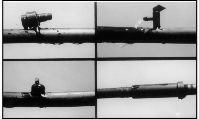
Figure 11. Examples of point source emitters
