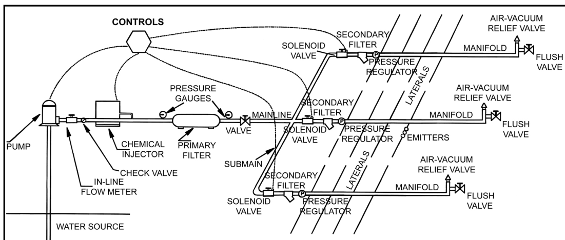
Figure 10. Components of typical drip irrigation system
