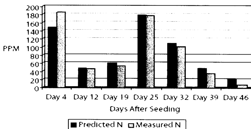
Figure 4-12. A comparison of predicted (based on conductivity) and measured nitrogen concentrations in a float bed, 2002
