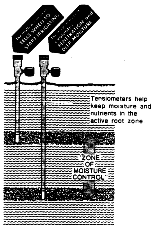
Fig. 2. Proper Use of Tensiometers
