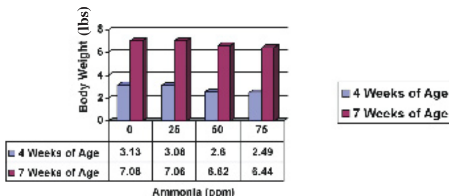
Figure 3. Exposure to ammonia concentrations as low as 25 ppm for the first 28 days can have a negative effect on body weight at both 4 and 7 weeks of age (Miles et al., 2004).
