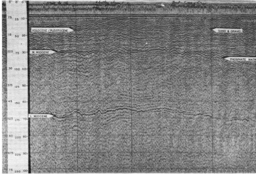
Plate 4 Seismic section, Ogeechee river abeam Rabbit Hill, extending W. (left) to E. (right).
