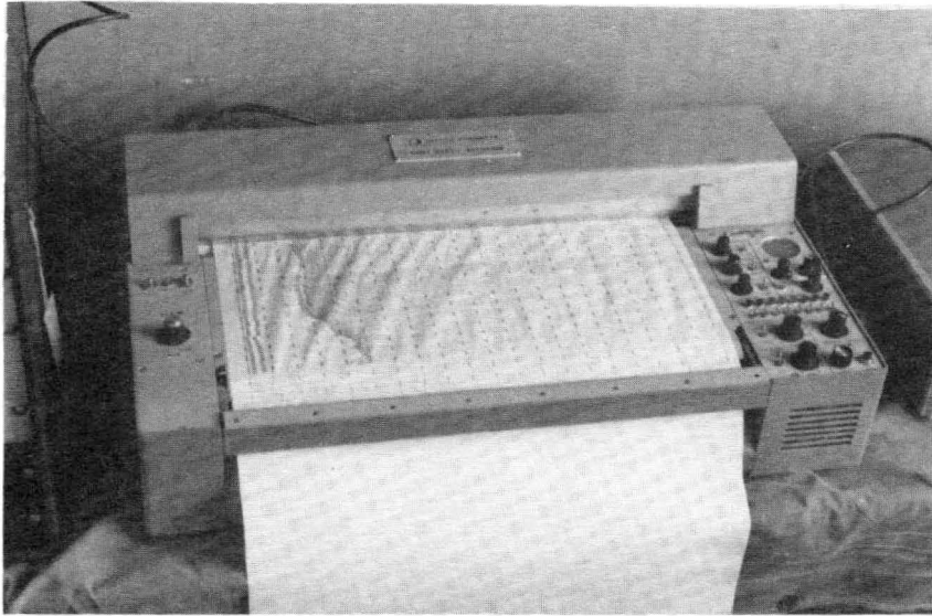
Plate 11 Seismic recorder with sub-bottom profile record.
