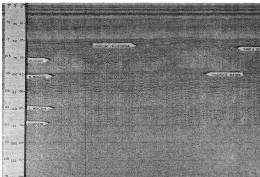
Plate 2 Seismic section, approximately 5 miles southeast of Little Tybee Island extending from S.W. (left) to N.E. (right), showing erosion surface (channel dissection) developed on Pliocene sediments.
