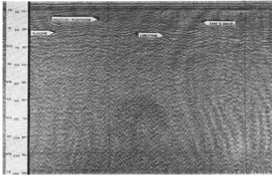
Plate 8 Seismic section, St. Mary's River, abeam Point Peter. Note shallow contact with Pliocene limestone; common to the south of the Little Satilla River.
