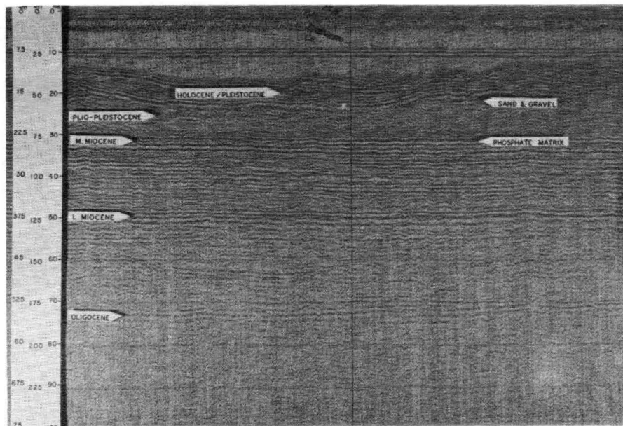
Plate 1 Seismic section, Tybee River at confluence of Lazaretto creek, extending from N. (left ) to S. ( right ).
