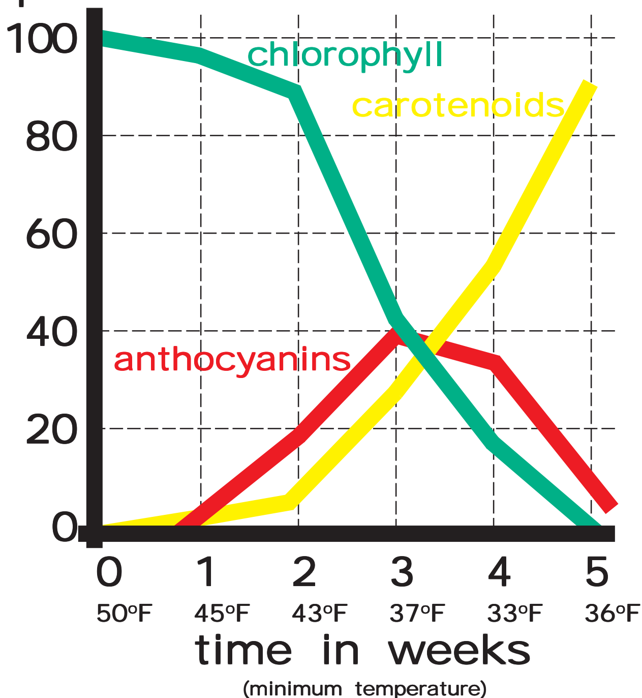
Figure 3: Relative color expression changes in sugar maple ( Acer saccharum ) trees in NE United States over one senescence period. (after Schaberg et.al. 2003)
