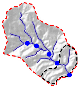
Figure 1-2. Segment center points (blue dots) were determined for each 2 nd order or larger stream. Drainage basins (red line) and “adjacent areas” (black line) were delineated for every segment center (though only illustrated here for the downstream-most segment).
