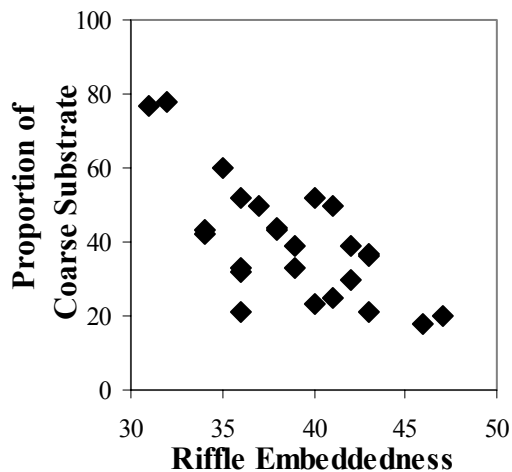
Figure 3-10. Proportion of coarse substrate related to riffle embeddedness. n = 25 ; r^2 = 0.49 ; p \text{ value} = 0.0001 . \text{Arcsine } (\% \text{ Coarse Substrate}^{0.5}) = (-0.028)(\text{Riffle Embeddedness Index}) + 1.796
