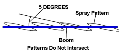
Figure 1. Flat fan nozzles angled 5 degrees from the boom.
