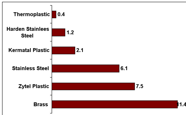
Figure 5. Percent increase to nozzle flow rate of flat fan spray.
