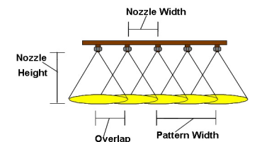
Overlap Nozzles 40-50 Percent
