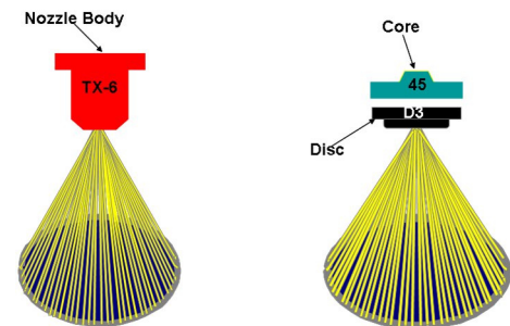
Figure 4. Hollow cone nozzles — nozzle body and disc-n-core
