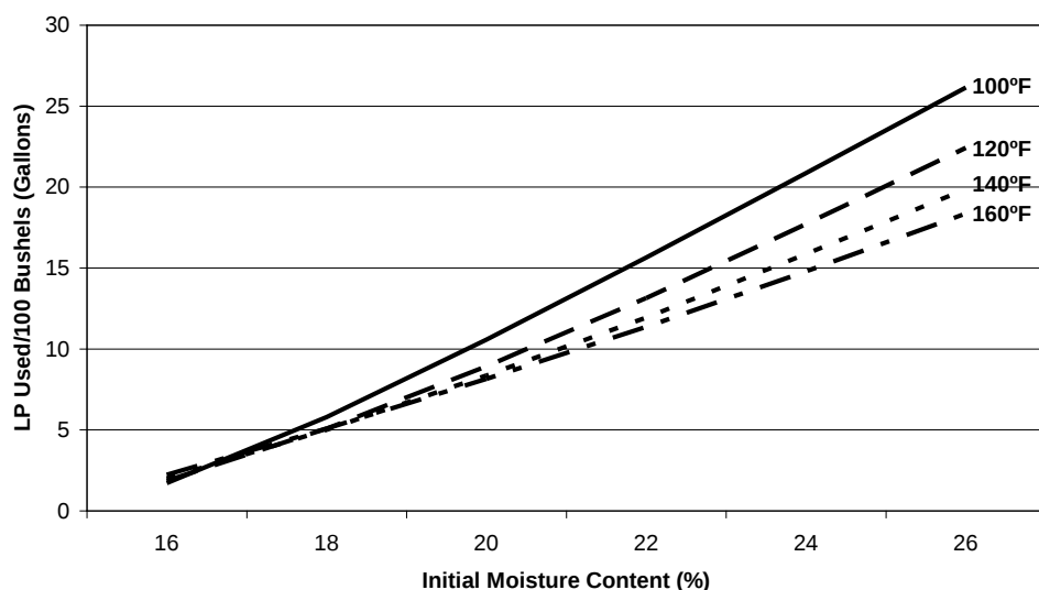
Figure 4. Estimated LP fuel use for corn with air at 85°F and 85 percent relative humidity, 30 CFM/Bushel, 50 CFM/ft 2 of floor area.
