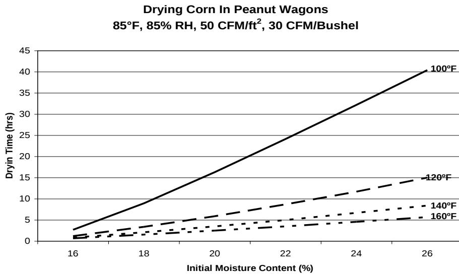
Figure 2. Estimated total drying time for corn with air at 85°F and 85 percent relative humidity, 30 CFM/Bushel, 50 CFM/ft 2 of floor area.
