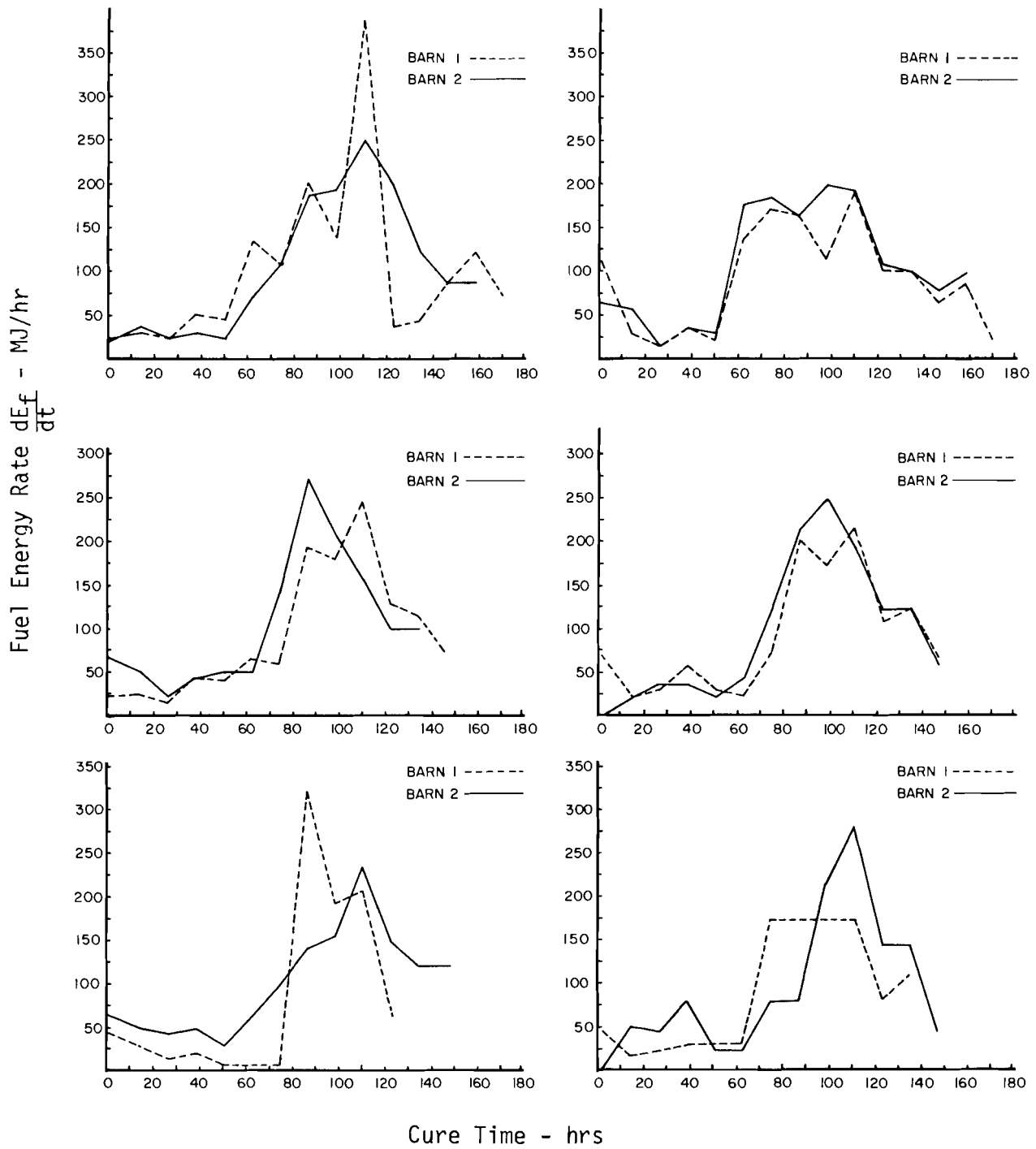
Figure 2. Fuel consumption rate for Barns 1 and 2, Cures 2-7 respectively.
