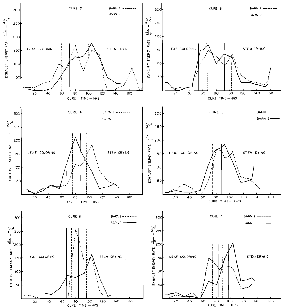
Figure 4. Exhaust energy rate for Barns 1 and 2, Cures 2-7 respectively.
