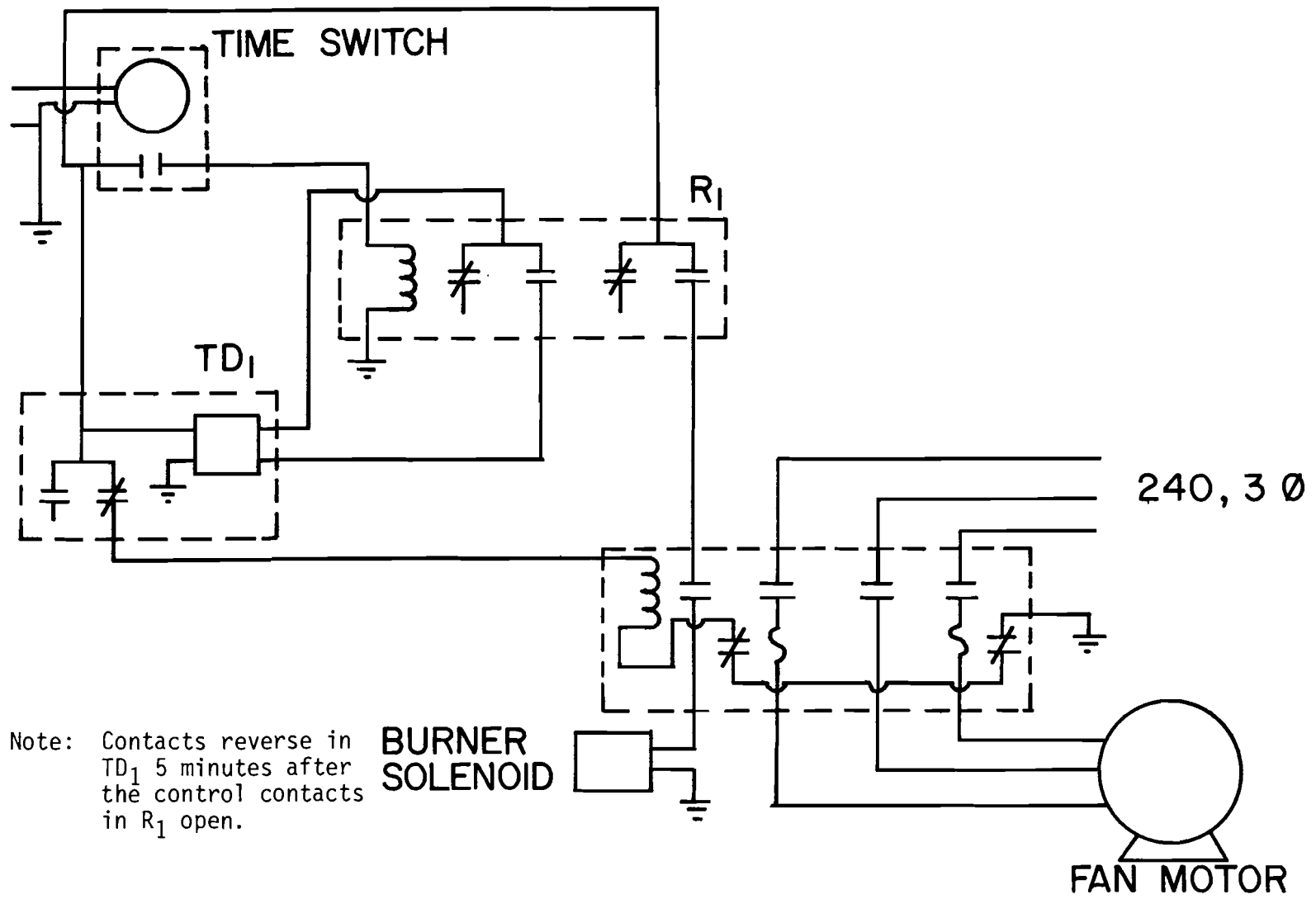
Figure 1. Control circuit for cycled barn (Barn 1).
