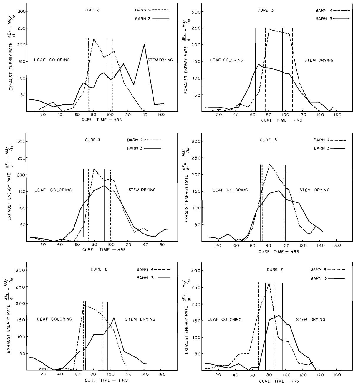
Figure 5. Exhaust energy rate for Barns 3 and 4, Cures 2-7 respectively.
