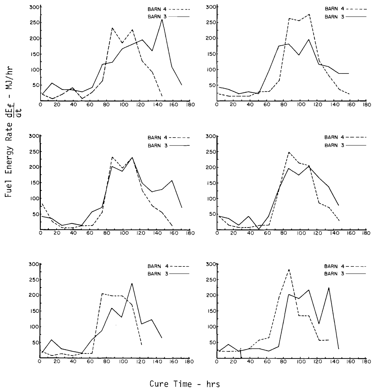
Figure 3. Fuel consumption rate for Barns 3 and 4, Cures 2-7 respectively.
