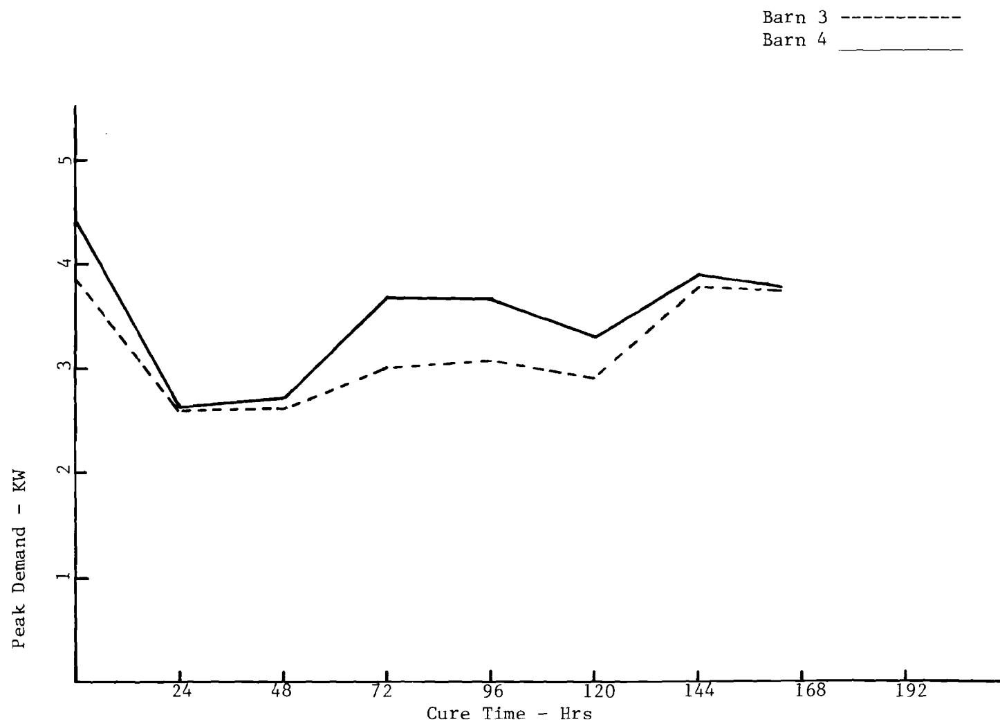
Figure 9. Peak Demand, (KW), for Barns 3 and 4, Cure 7.
