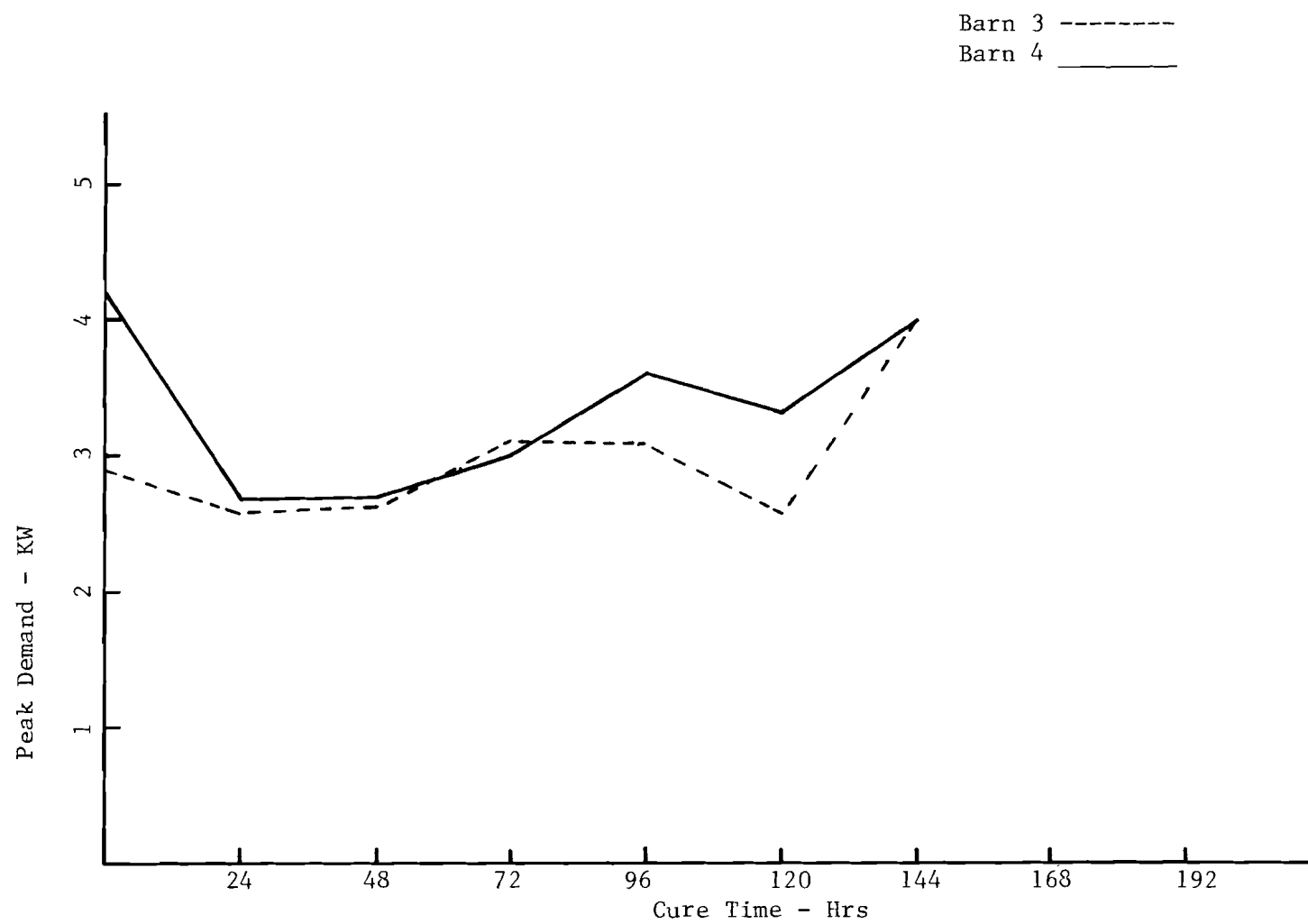
Figure 7. Peak Demand, (KW), for Barns 3 and 4, Cure 5.
