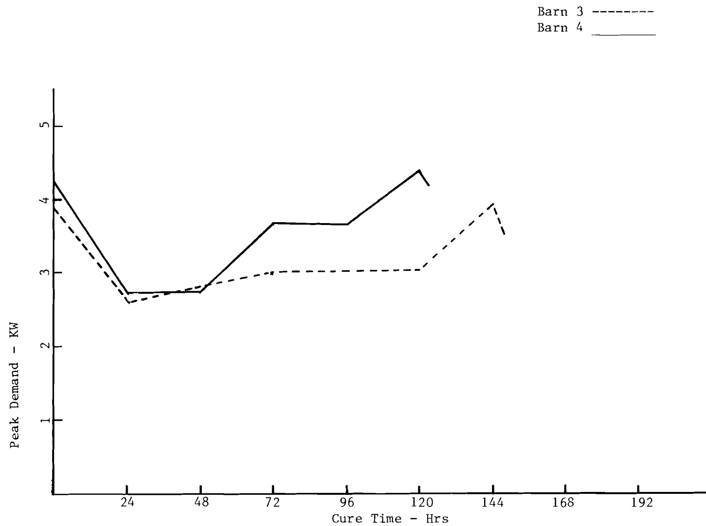
Figure 8. Peak Demand, (KW), for Barns 3 and 4, Cure 6.
