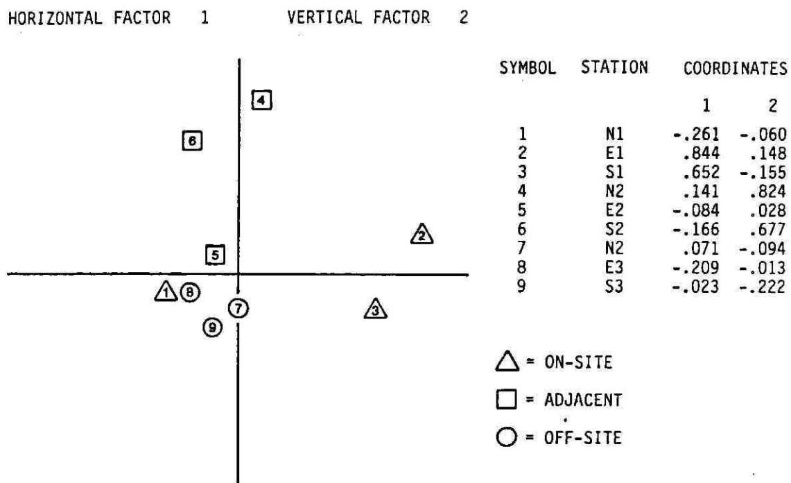
Figure Va. PCA plot for October, 1984 box core macroinfauna stations. Shapes associated with symbols indicate location relative to the dredge spoil disposal site.
