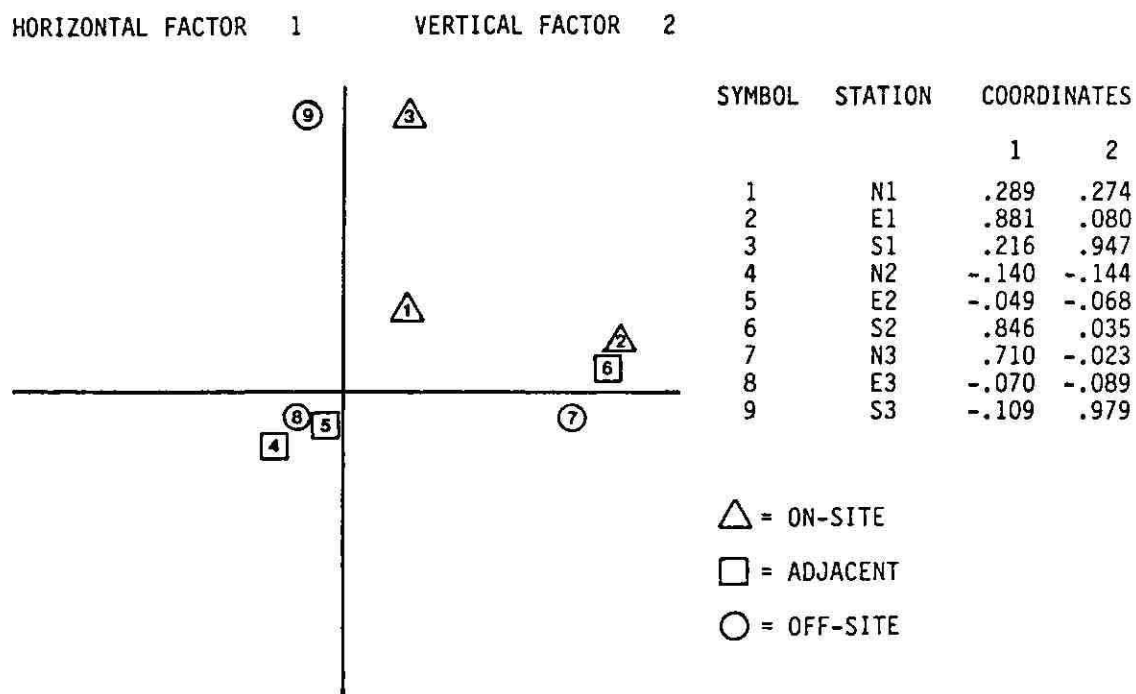
Figure Vb. PCA plot for April, 1985 box core macroinfauna stations. Shapes and symbols as in Fig. Va.
