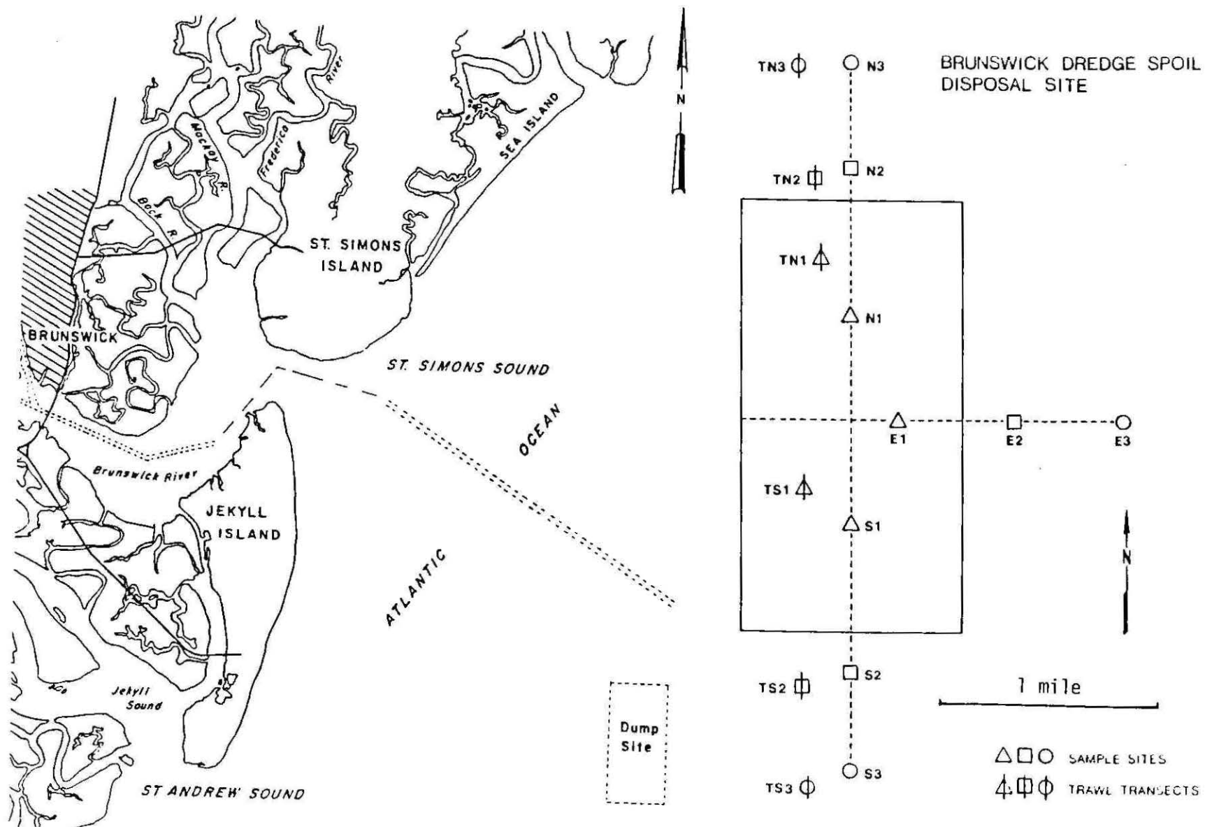
Figure 1. Sample locations in the Brunswick, Georgia dredge spoil ocean disposal site. Locations are approximate.
