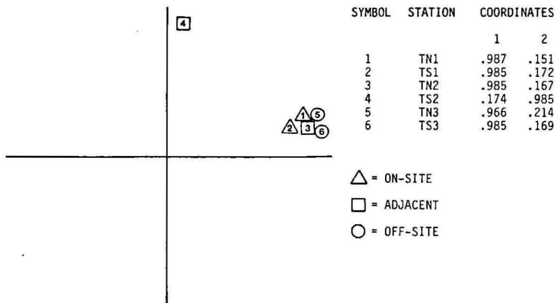
Figure IIIb. PCA plot for April, 1985 trawl macrofauna stations. Shapes and symbols as in Fig. IIIa.
