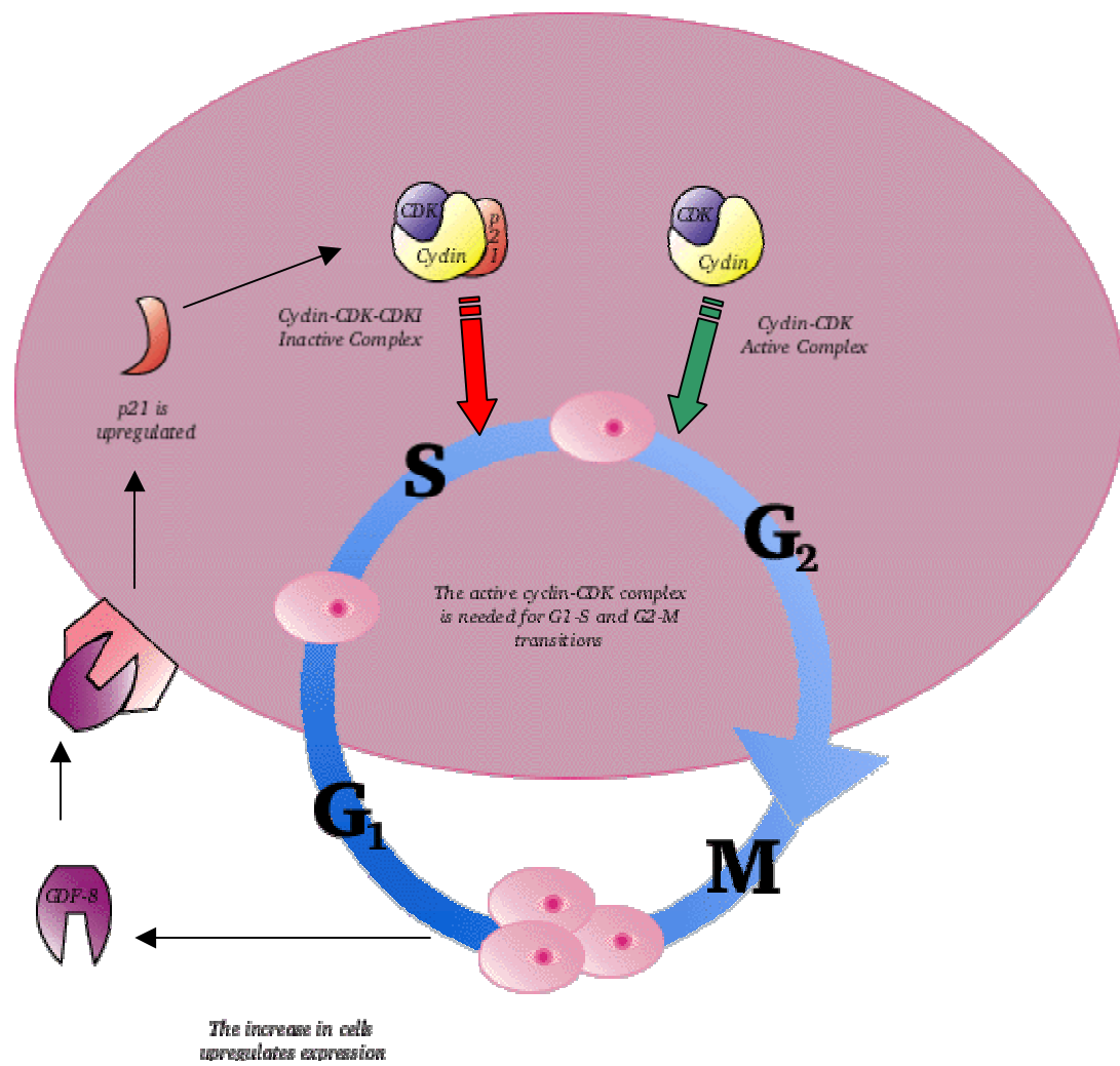
Figure 10: Myostatin mechanism
