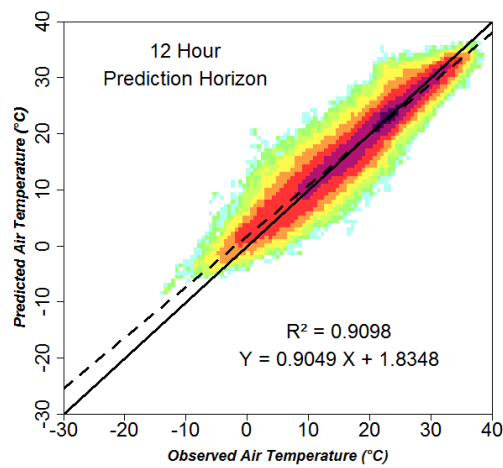
Figure 5. Predicted and observed air temperature, combined model, model evaluation dataset.
