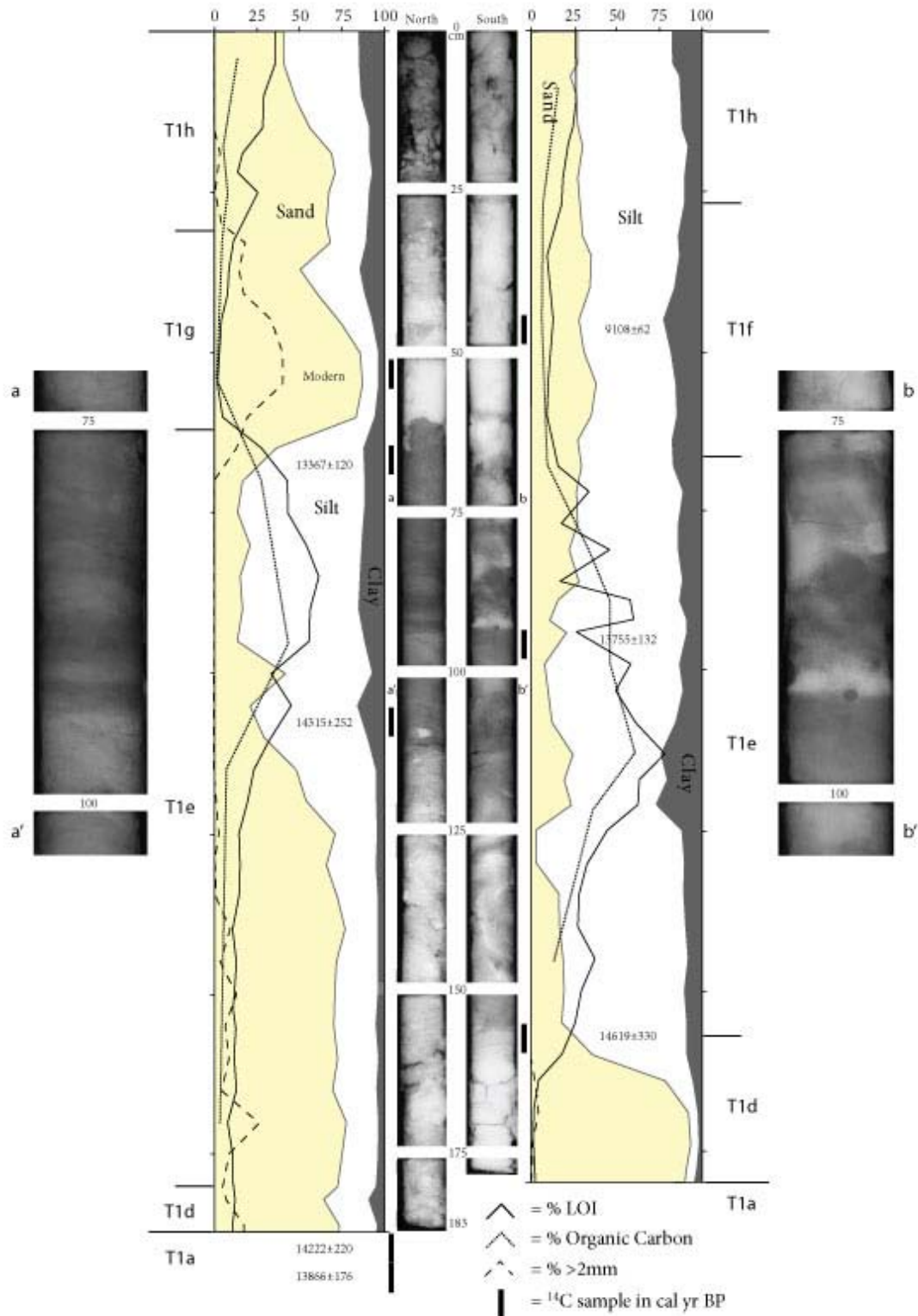
Figure 6 – Laboratory results. (PSA, LOI, x-ray, organic carbon, and radiocarbon dating) Stratigraphic units are also listed to provide easier interpretation. A zoomed in view of the inorganically bedded portion of T1e is shown to the left and right of the cores.
