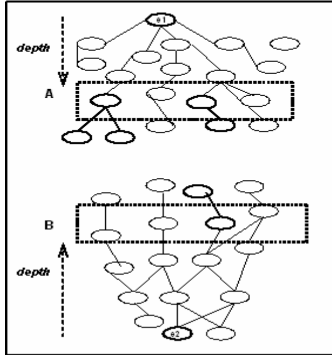
Figure 5.6 Interactive Deepening
