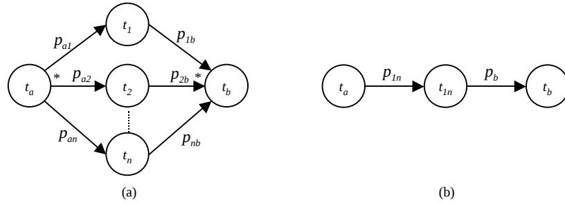
Figure 2-4 - Parallel system reduction
