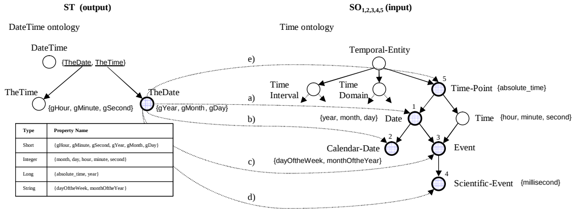
Figure 4-7 – Comparing proprieties referencing primitive data types
