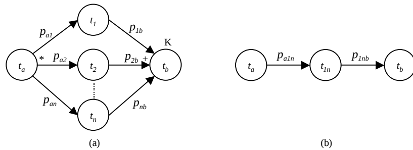
Figure 2-8 – Fault-Tolerant system reduction
