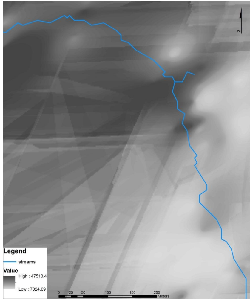
Figure B.2.7. Kriged map of C (0-7.5cm) (kg/ha), using above semivariogram. RMSE = 6773.48. Avg. Standard Error = 0.4246.
