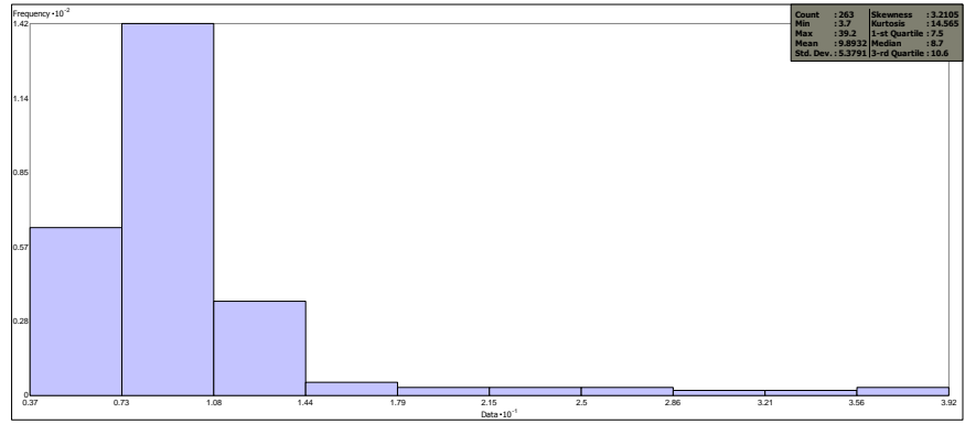
Figure B.6.4. Silt frequency distribution.
