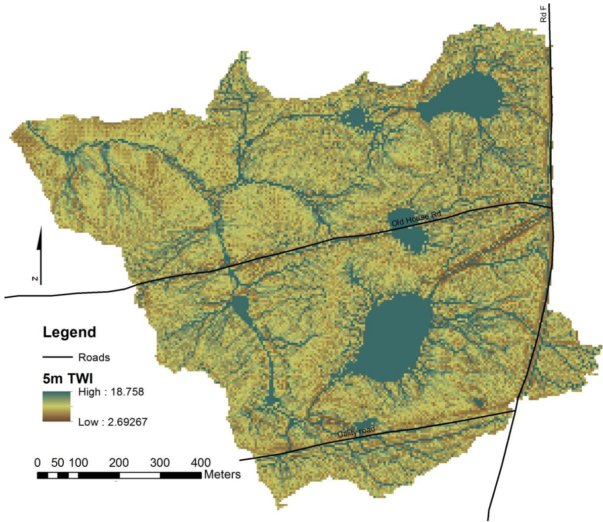
Figure 3.4.5. Map of 5m TWI in basin C.
