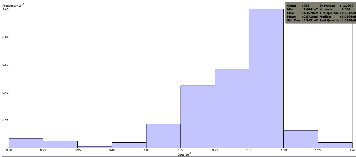
Figure B.5.5. Box-Cox-transformed ( \lambda=5 ) sand frequency distribution.
