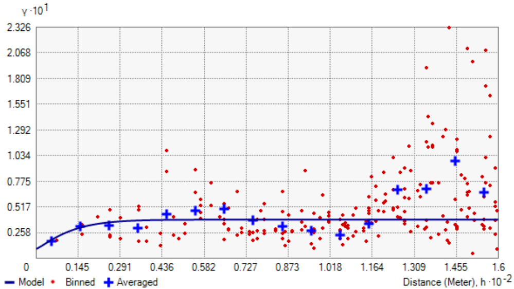
Figure B.7.6. Semivariogram for bulk density. The major axis is 160m, minor axis is 120m and the direction is 122.5°
