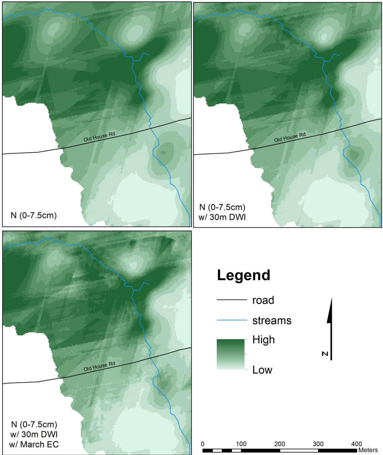
Figure 4.3.9. Spatial distribution of N (0-7.5cm) values alone (top left), cokriged with 30m DWI (top right), and cokriged with 30m DWI and March EC (bottom left).
