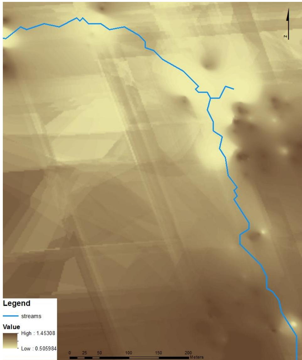
Figure B.7.7. Kriged map of bulk density ( \text{g}/\text{cm}^3 ), using semivariogram from figure B.7.6. RMSE = 0.1374.
