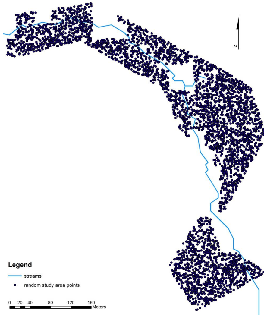
Figure 4.2.1. Random points generated for the study area. Each point was given a TWI, DWI and elevation value extracted from each resolution of its respective raster grid (total of 15 values per point). These were used for cokriging with soil attributes to improve predictions.
