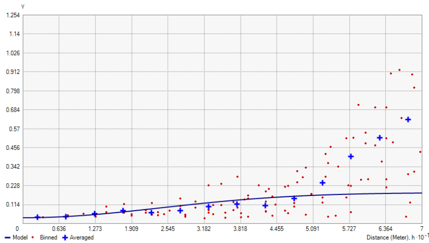
Figure B.6.6. Semivariogram for sand. The major axis is 70m, minor axis is 20m and the direction is 26.8°
