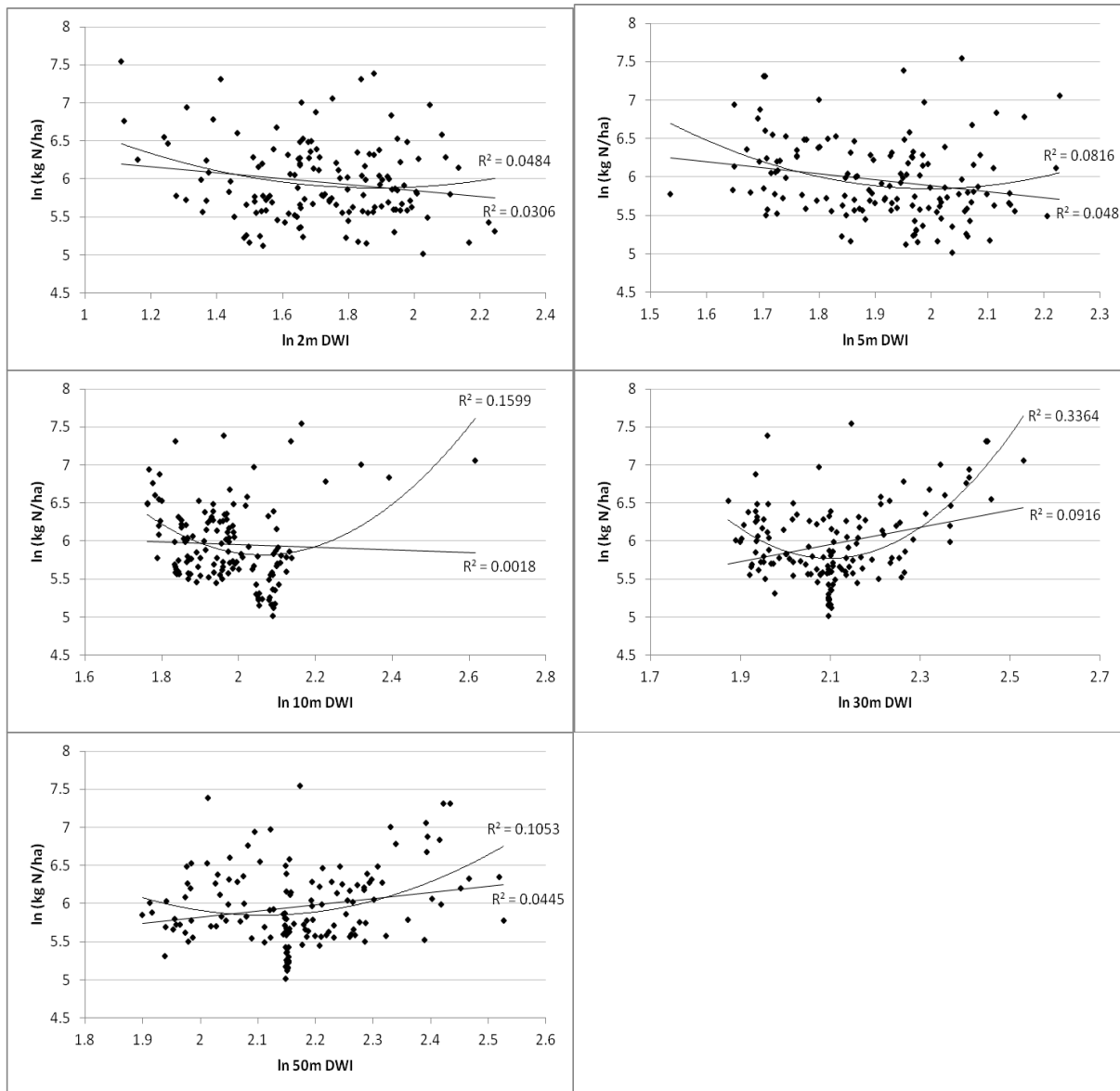
Figure 3.4.17. Linear and non-linear fits for DWI vs. N (0-7.5cm) at 2m, 5m, 10m, 30m, and 50m resolutions in the C basin. Note that the non-linear fit shows higher coefficient of determination and improves homoscedasticity (n=142).
