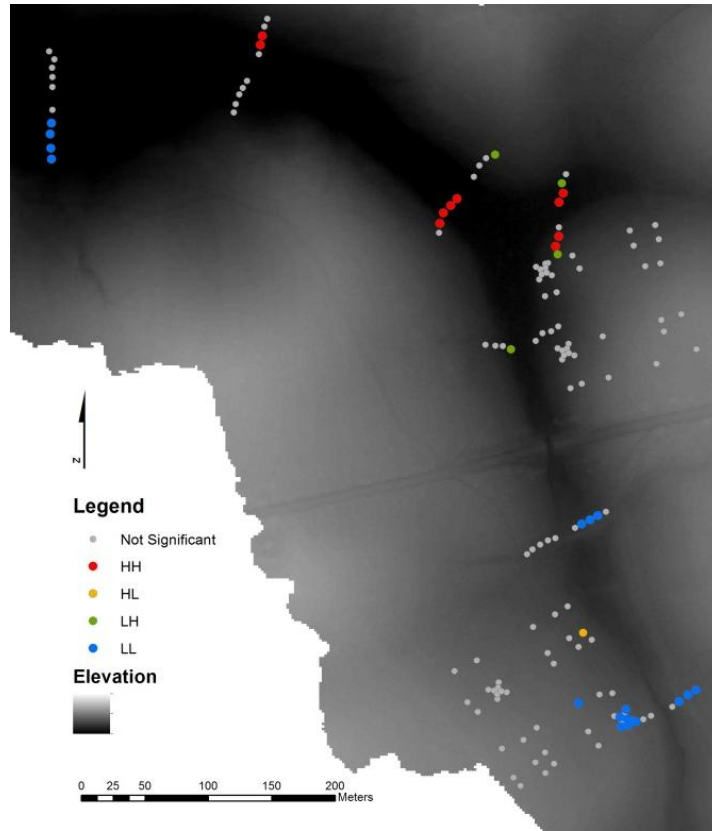
Figure B.8.2. Local Moran's I map, showing significant ( p < 0.05 ) clustering of high and low values of A horizon thickness. HH and LL stand for high and low clustering, respectively. HL and LH stand for high values surrounded by low values and low values surrounded by high values, respectively.
