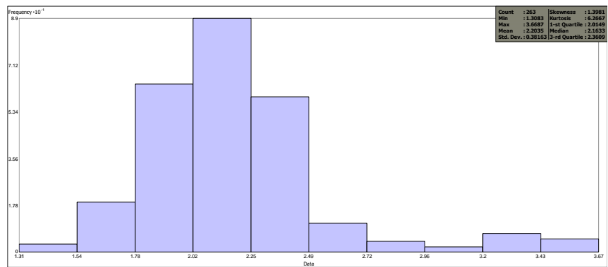
Figure B.6.5. Log-transformed silt frequency distribution.
