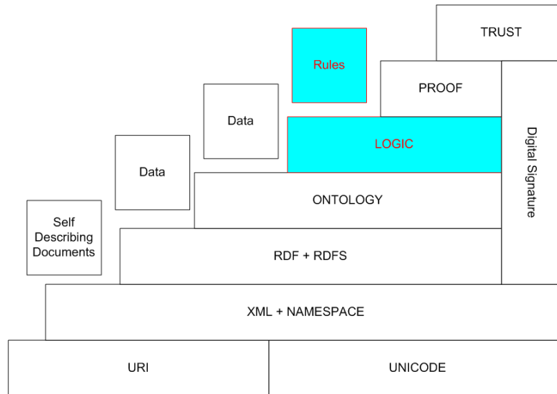
Figure 2: Semantic Web Stack
