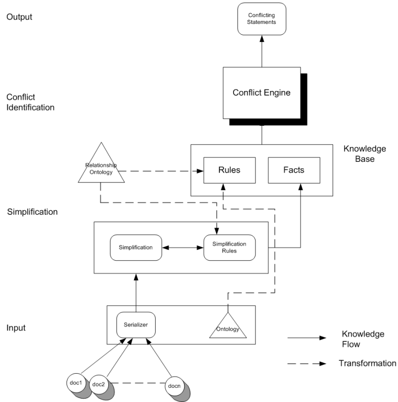
Figure 9: Overview of System Architecture
