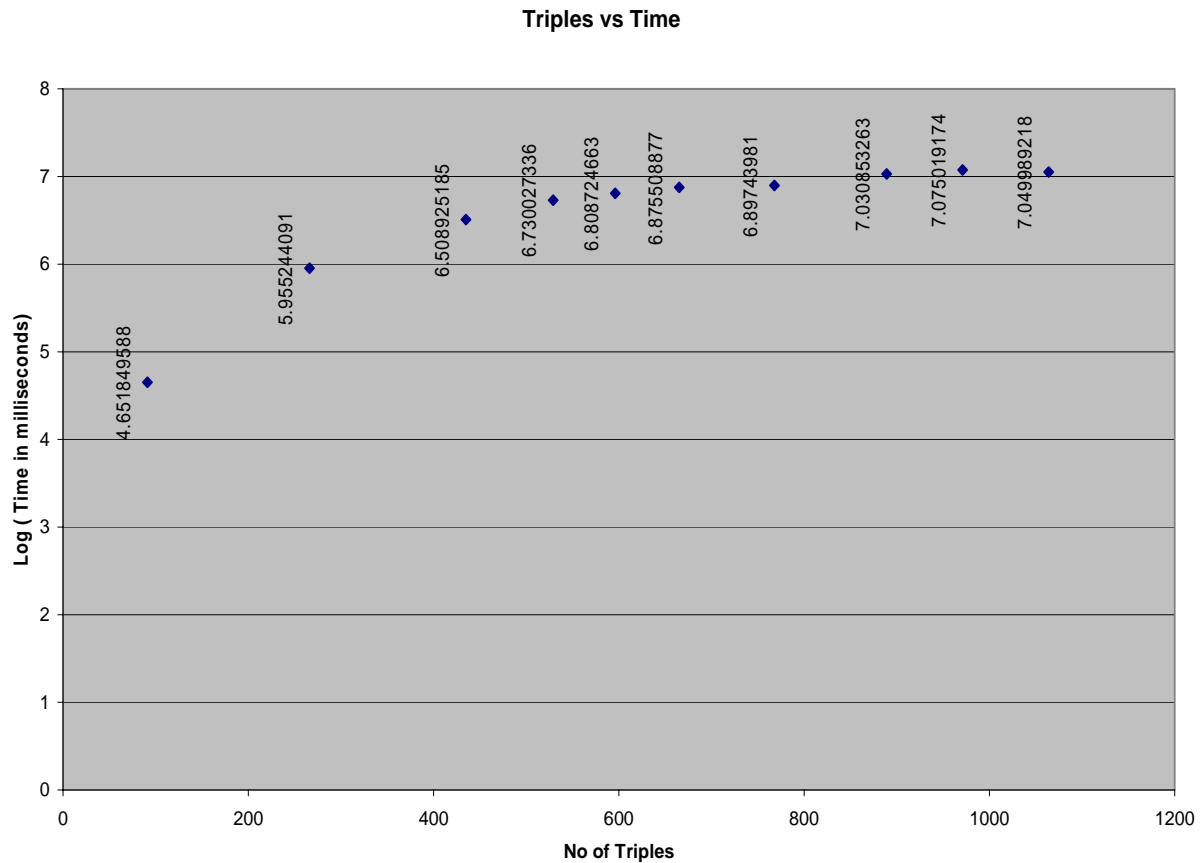
Figure 13: Performance with increase in number of triples (10 conflicts)
