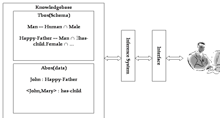
Figure 7: Description Logic Based System
