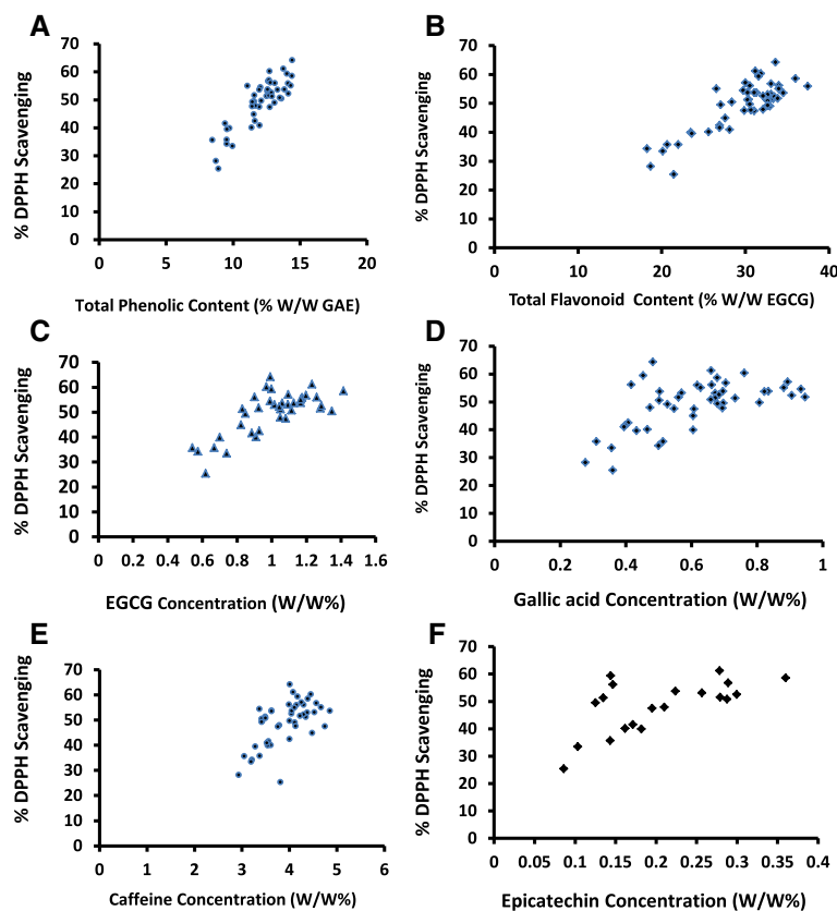
Fig. 4 Correlation of antioxidant activity with the concentration of polyphenols (a), flavonoids (b), EGCG (c), gallic acid (d), caffeine (e) and EC (f)
