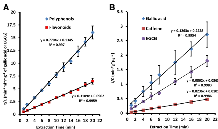
Fig. 1 Correlation between t/C and extraction time for polyphenols and flavonoids (a) and correlation between t/C and extraction time for gallic acid, caffeine and epigallocatechin gallate (b)
